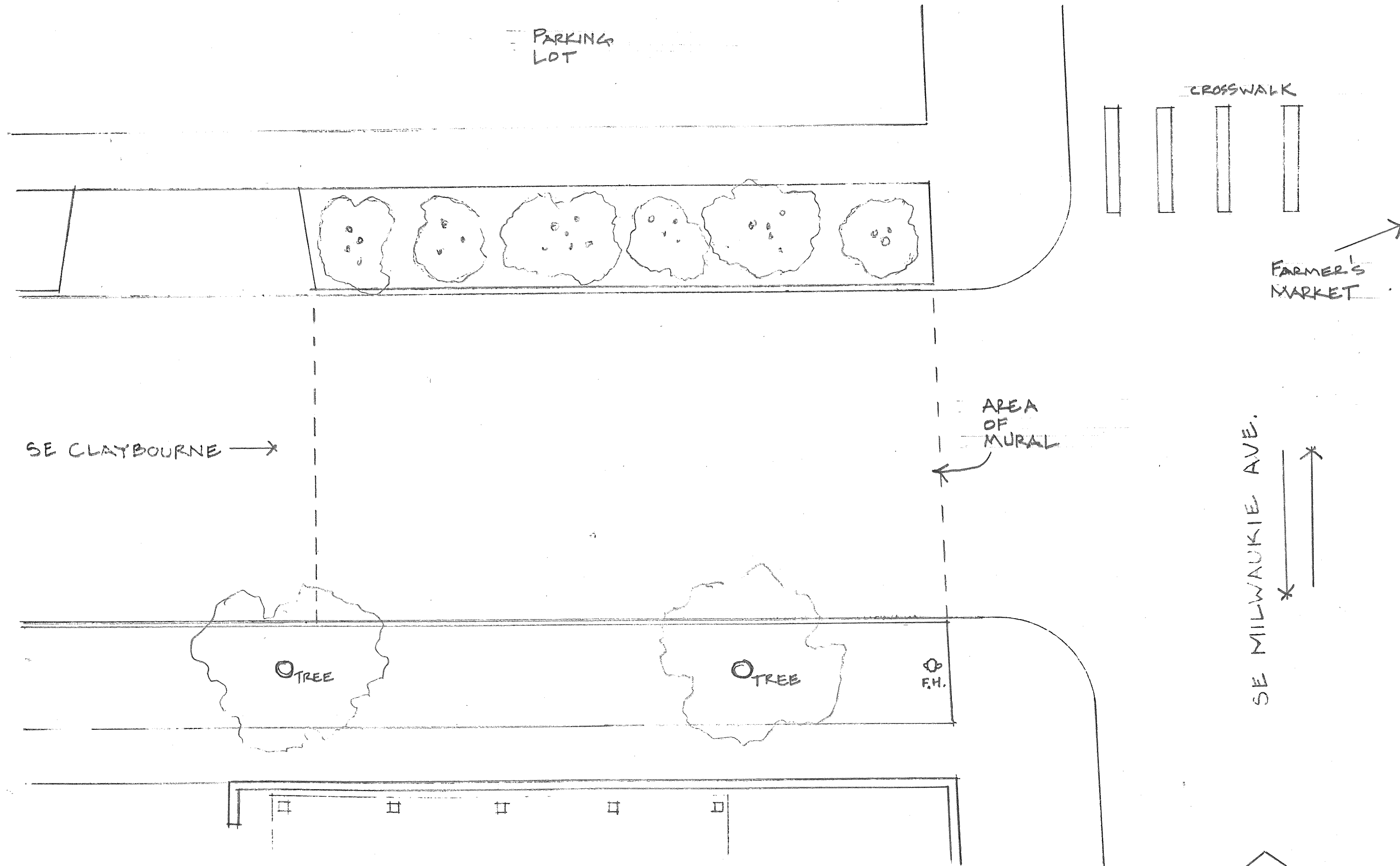
SE CLAYBOURNE PLAZA, STREET GRAPHIC BASE PLAN
